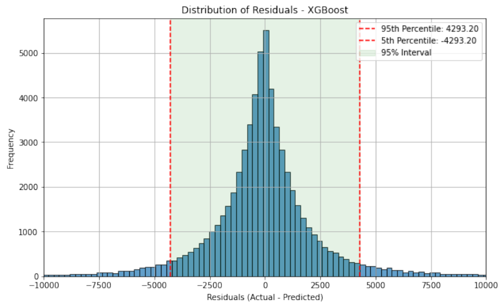
Figure 23: Residuals Distribution - Harshly Cleaned. Source: Own work
