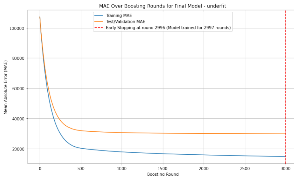
Figure 10: XGBoost Training MAE Curve. Source: Own work
