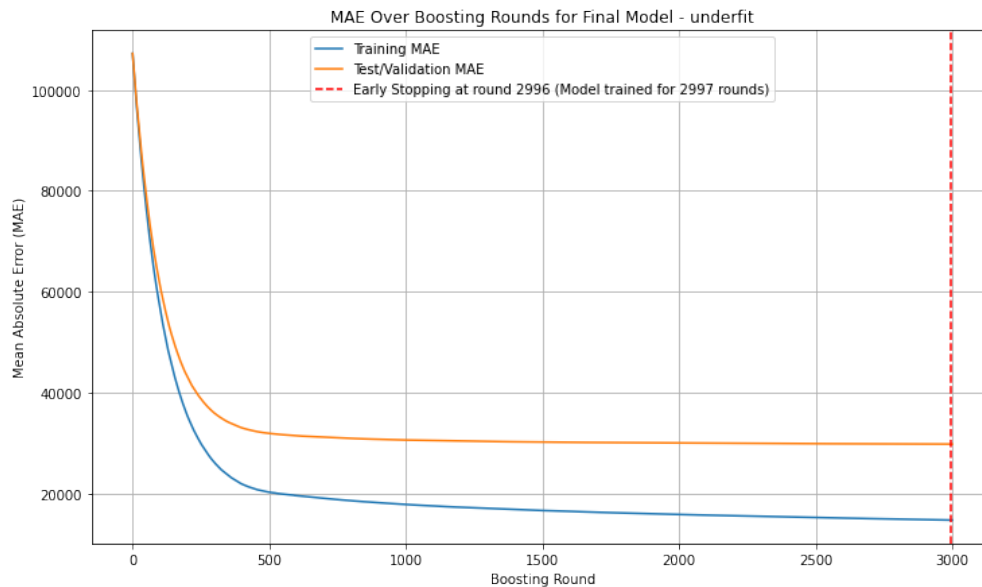
Figure 9: XGBoost Training MAE Curve. Source: Own work
