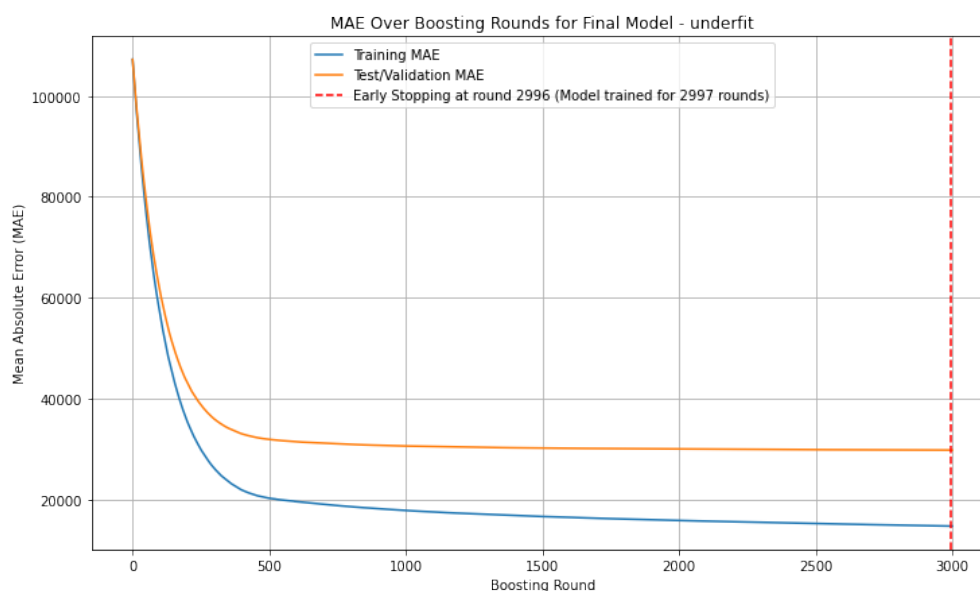
Figure 12: XGBoost Training MAE Curve. Source: Own work
