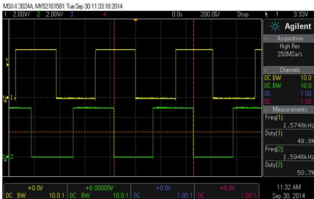
Encoder A and B outputs of a magnetic encoder on a high-power (HP) 6V Micro Metal Gearmotor running at 6 V.
