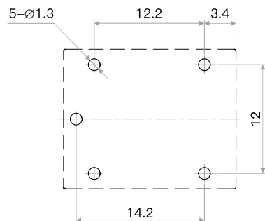
安装孔图(底视图)/Installation hole drawing(Bottom view)
