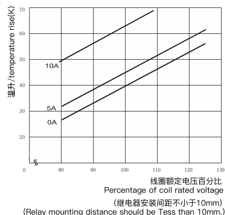
线圈温升 Coil temperature rise
