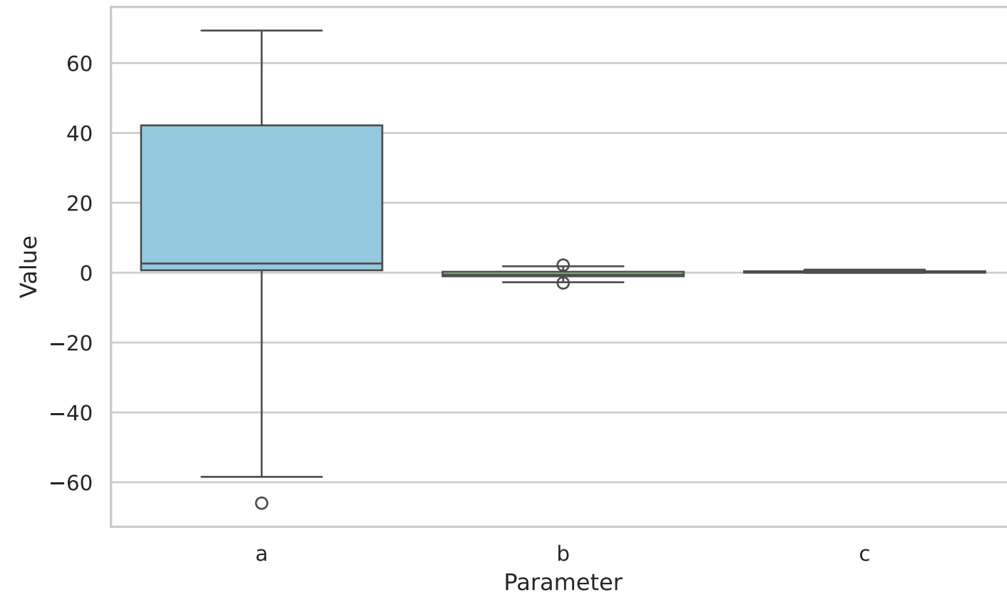
Box Plot of All Parameters
