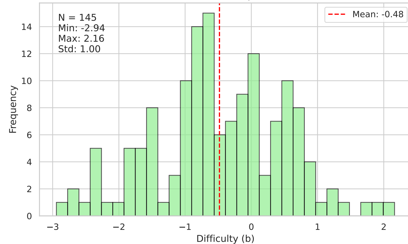
Distribution of Difficulty Parameters
