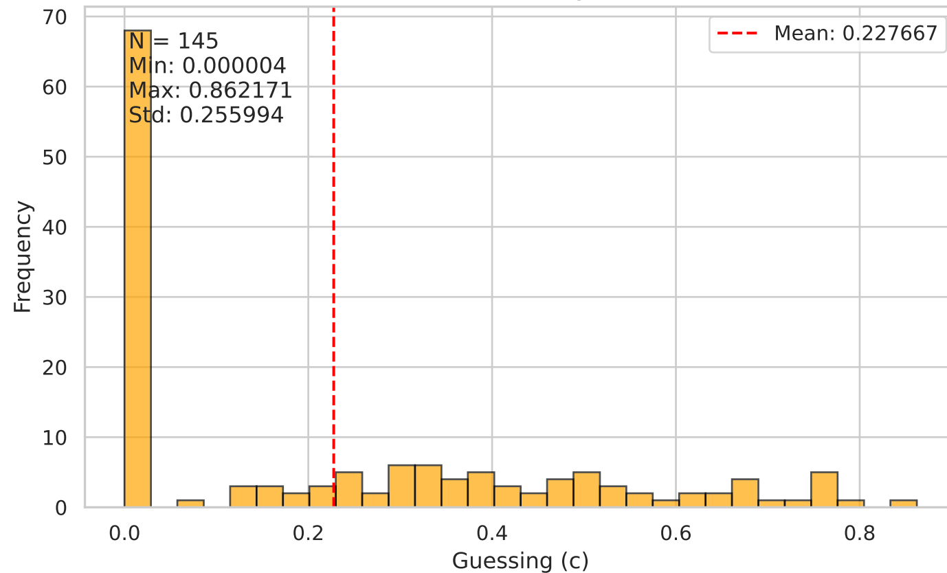
Distribution of Guessing Parameters
