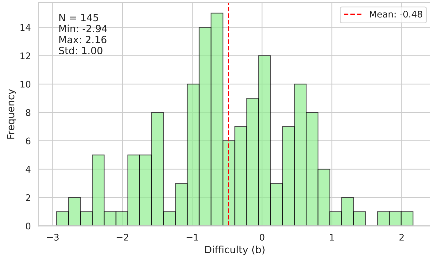
Distribution of Difficulty Parameters
