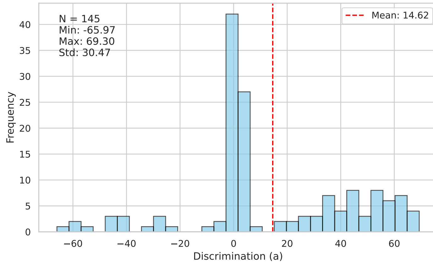
Distribution of Discrimination Parameters
