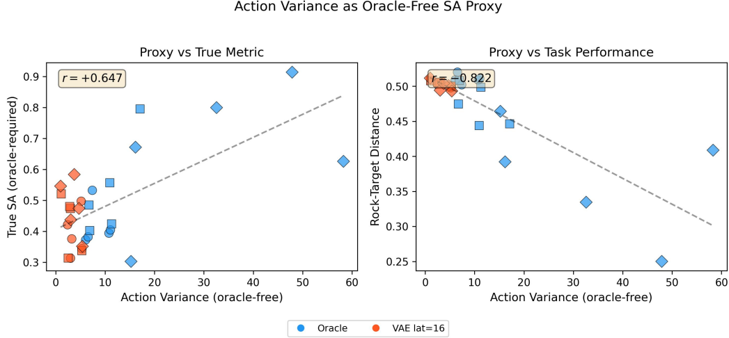
Figure 3: Action variance as an oracle-free SA proxy. (a) Action variance vs. true SA ( r = +0.65 ). (b) Action variance vs. task performance ( r = -0.82 ), comparable to true SA’s r = -0.80 . Oracle-free, computable from policy outputs alone.
