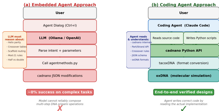
Figure 1: Architecture comparison. (a) Embedded tool-using LLM achieved 0% success on multi-step design tasks because the model could not resolve contextual constraints (helix parity, crossover directionality) from tool schemas alone. (b) Coding agent with source code access produced end-to-end verified designs by reading cadnano internals, writing Python scripts, and integrating external simulation tools.
