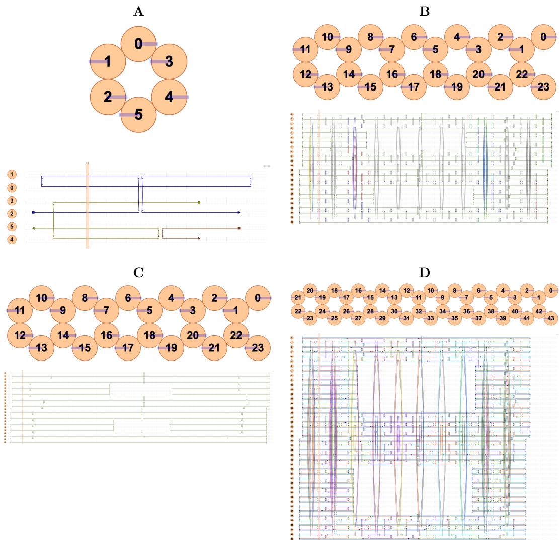
Figure 4: Formalizing cavity design. Slice view (top) and path view (bottom) for each panel. (A) Agent's initial attempt at scaffold routing: disconnected oligos. (B) User-provided template showing scaffold routing with cavity gap (staples hidden for clarity), 1 scaffold oligo (5,036 bp). The routing changes at the cavity boundaries: half-crossovers serve as scaffold turns, while full crossovers connect the interior. (C) Correctly routed 30 nm cavity design with 1 scaffold oligo, produced by the agent after incorporating the user's corrections. (D) Final stapled product after autoStaple + autoBreak (220+ staples, minLegLen=3), ready for tacoxDNA conversion and oxDNA molecular dynamics simulation.
