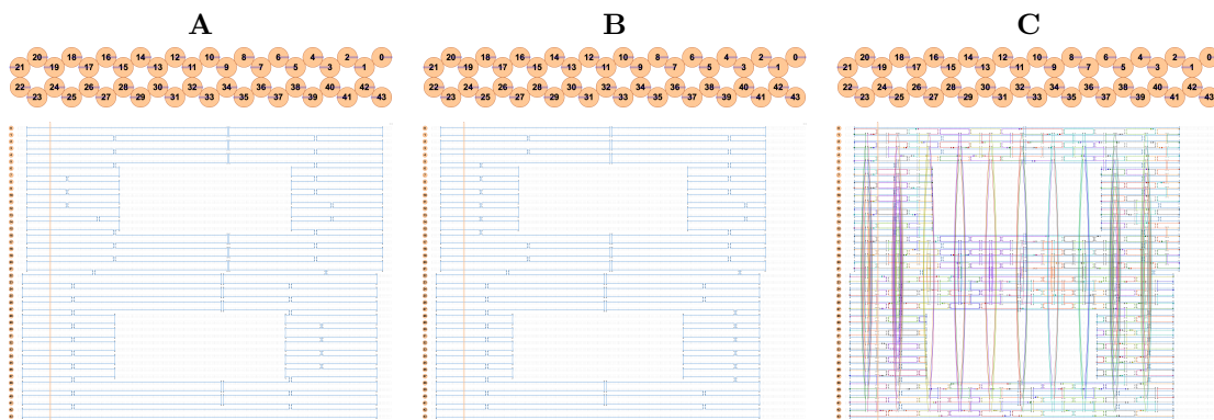
Figure 5: One-shot targeted edits on the 2-by-22 integrin cavity design. Slice view (top) and path view (bottom) for each panel. (A) Starting state: scaffold-only, before edits. (B) After two edits: structure shrink (edge crossovers moved inward, 252 \rightarrow 225 bp) and crossover repositioning + cavity centering (5 inter-pair crossovers moved 26+ bp from cavity boundaries, cavity centered to within 1 bp). (C) After autoStaple + autoBreak (220+ staples, minLegLen=3): complete stapled design ready for tacoxDNA conversion. Each edit executed correctly on the first attempt.
