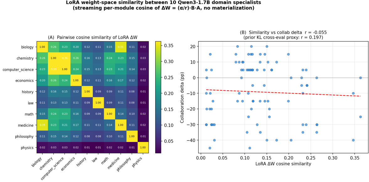
Figure 4: LoRA weight-space similarity across 10 Qwen3-1.7B specialists. (A) Pairwise cosine similarity matrix of \Delta W = (\alpha/r) \cdot B \cdot A per module, averaged across modules. (B) Similarity vs collaboration delta across 90 ordered pairs; r = -0.055 , no linear signal.
