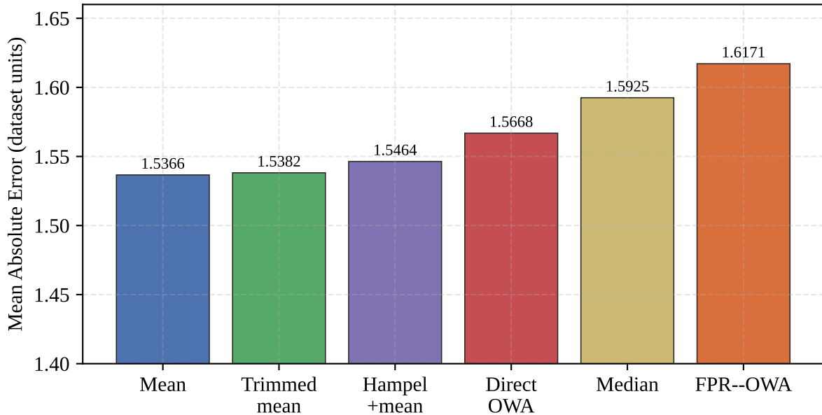
Global MAE by consensus method (1890 scenarios)
