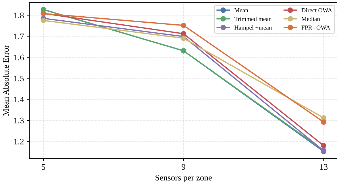
Effect of sensor redundancy on consensus accuracy
