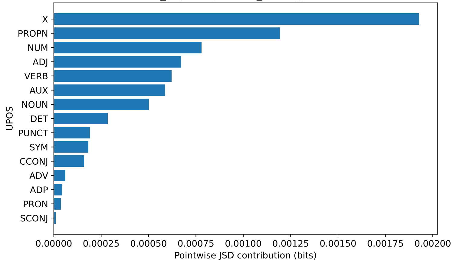
arxiv_papers: gemma2_9b vs gpt-4o-mini
