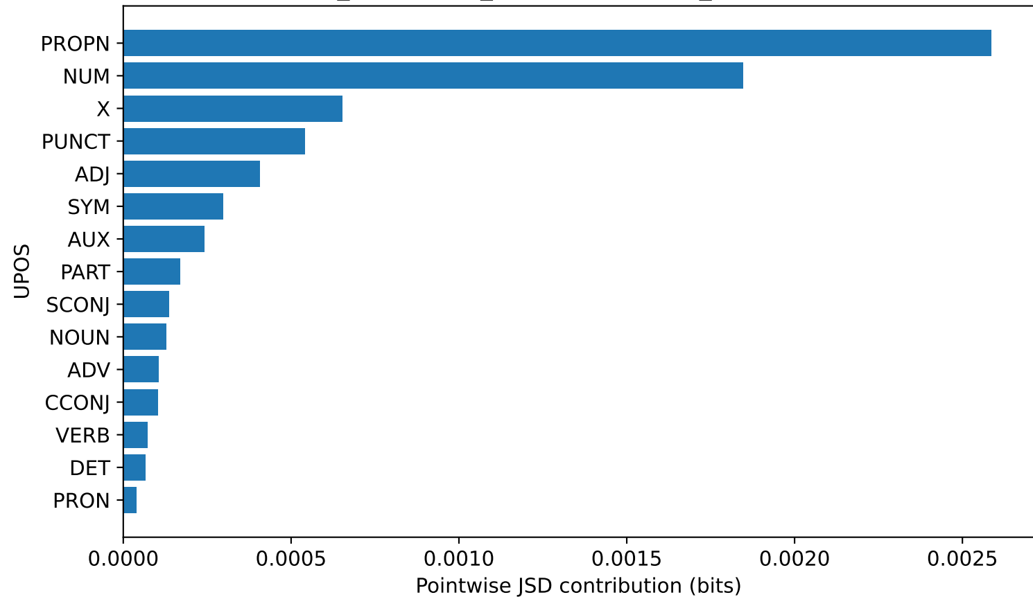
blog_authorship_corpus: gemma2_9b vs human
