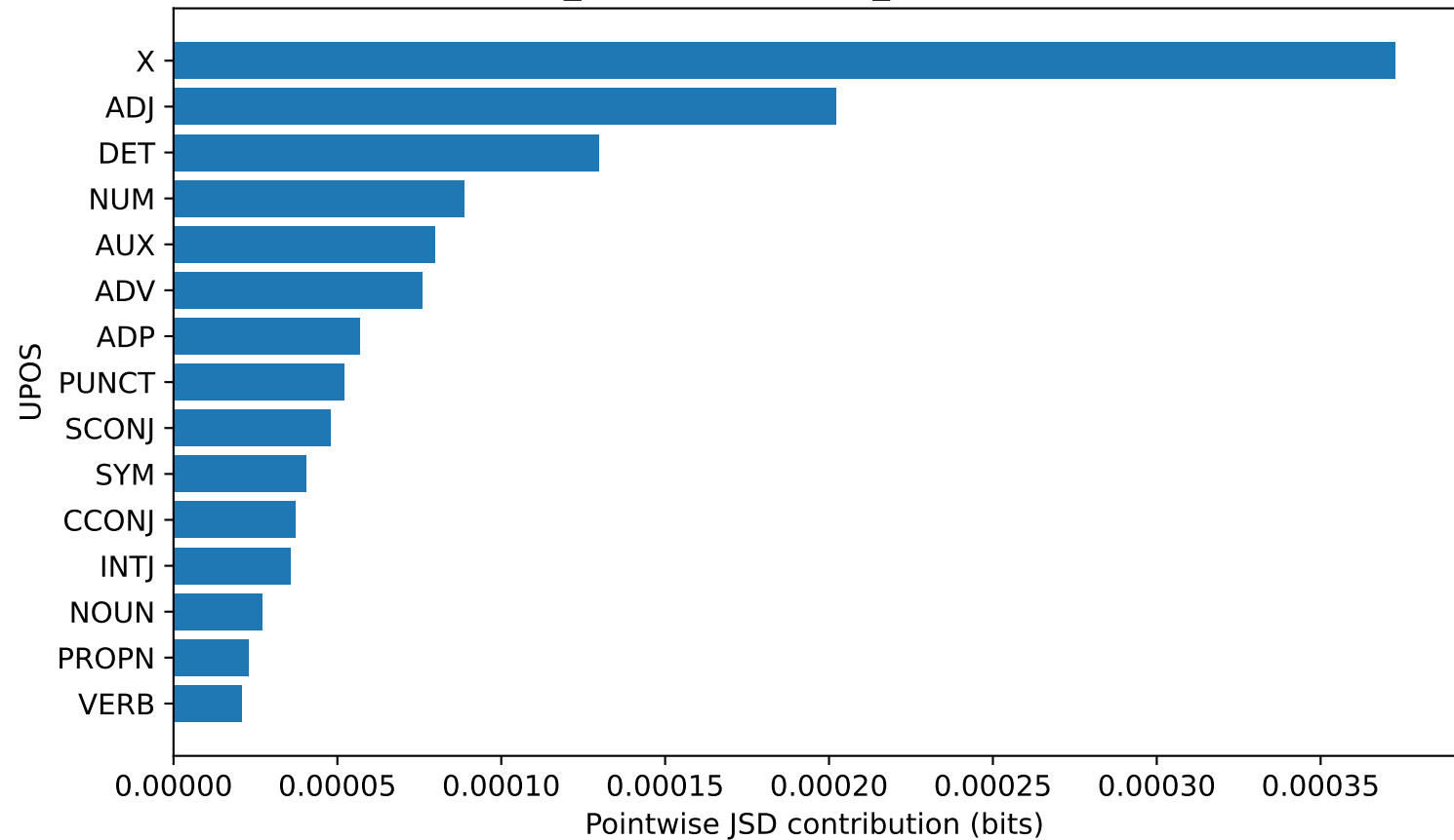
student_essays: gemma2_9b vs gpt-4o-mini
