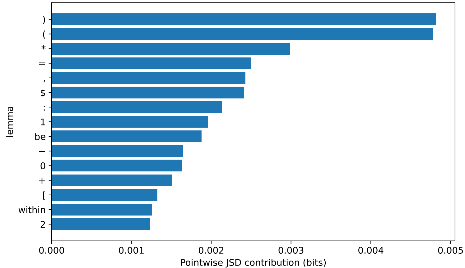
arxiv_papers: gemma2_9b vs human
