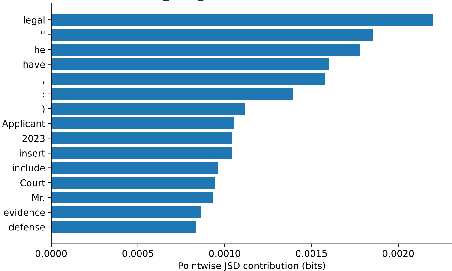
euro_court_cases: gpt-4o-mini vs human
