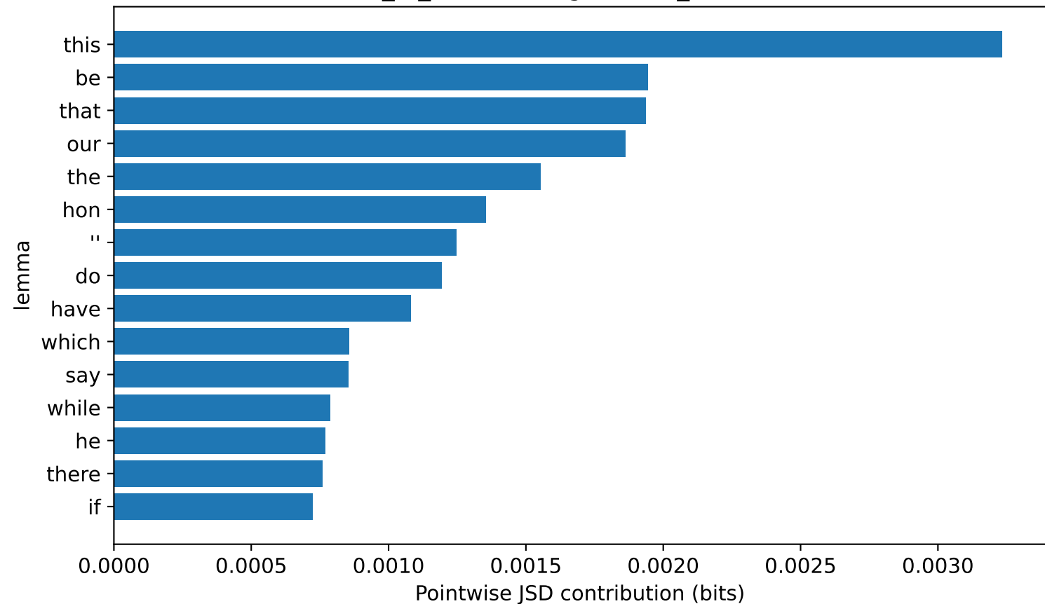
house_of_commons: gemma2_9b vs human
