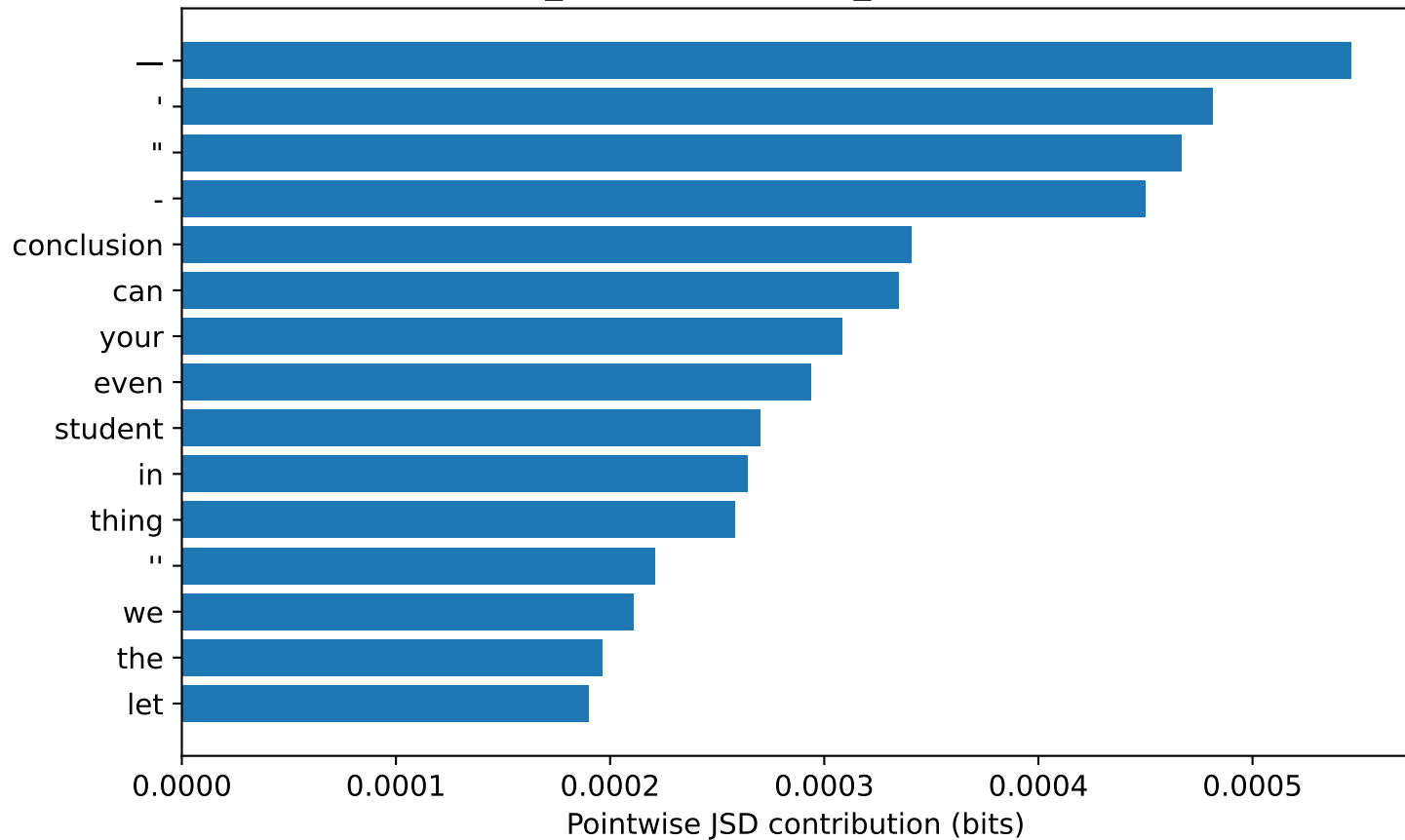
student_essays: gemma2_9b vs gpt-4o-mini
