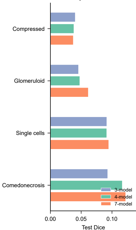
a Rare-specialist ensembles
