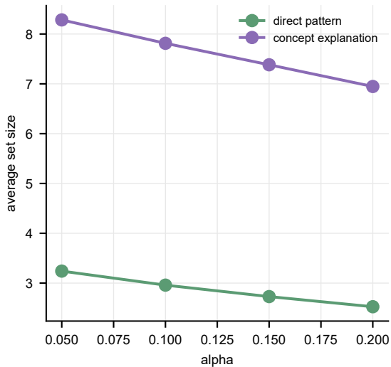
b) prediction-set size
