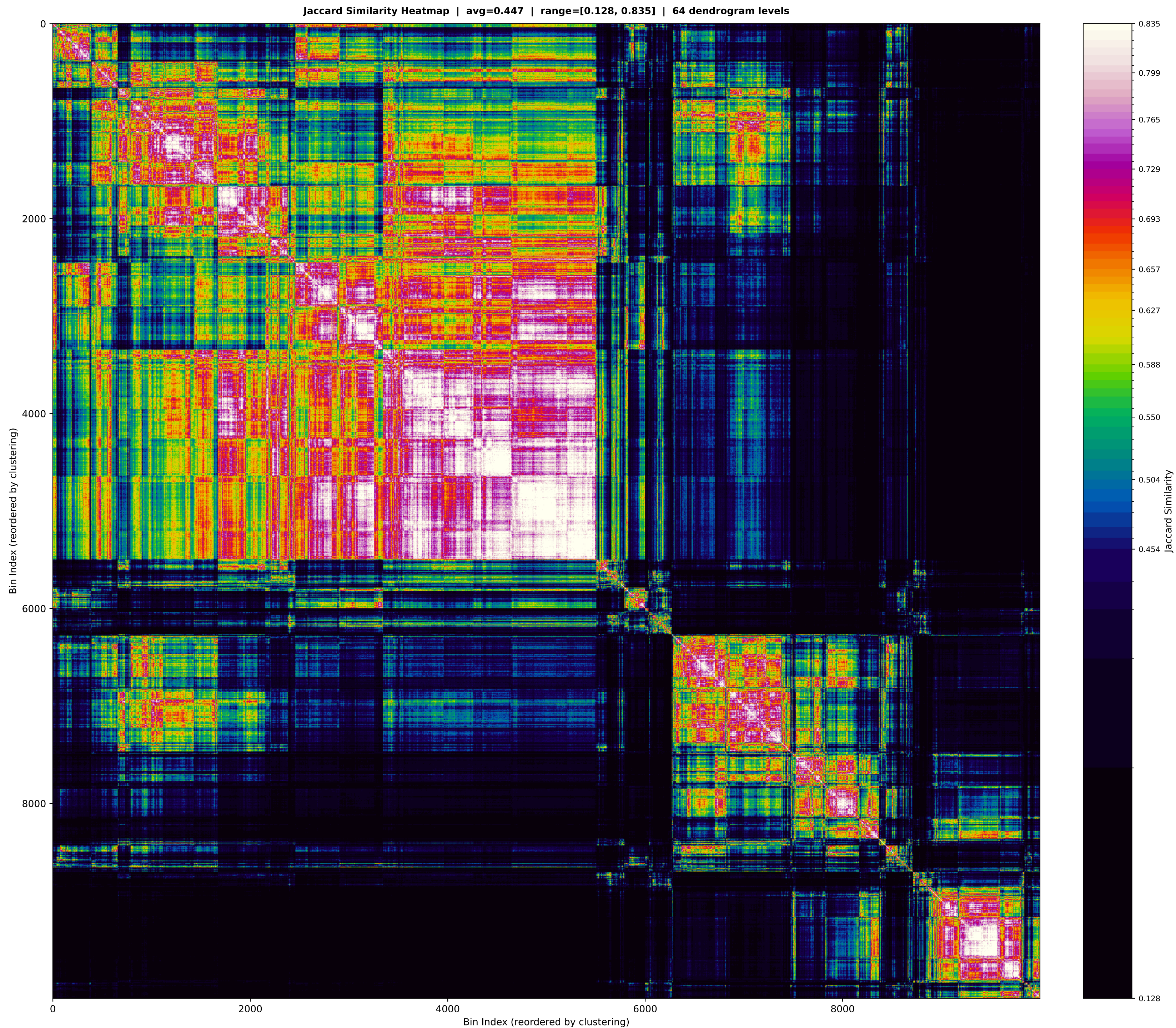
Hierarchical Clustering (10,000 bins, 30,000 samples)
