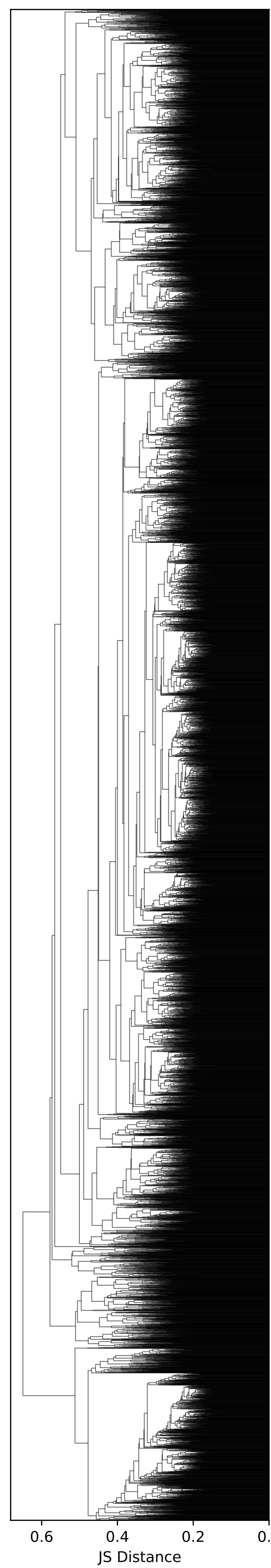
Hierarchical Clustering (10,000 bins, 30,000 samples)
