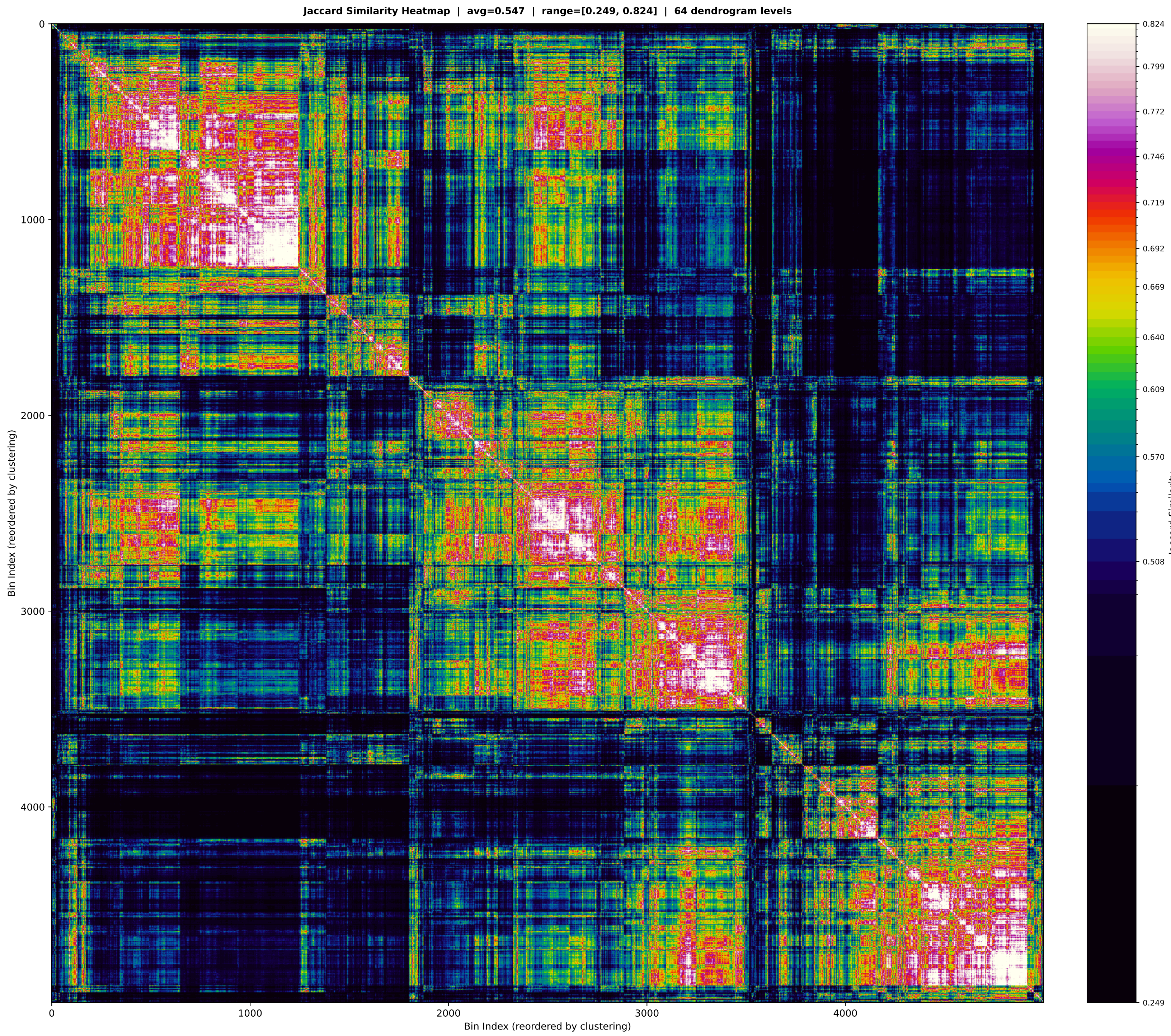
Hierarchical Clustering (5,000 bins, 30,000 samples)
