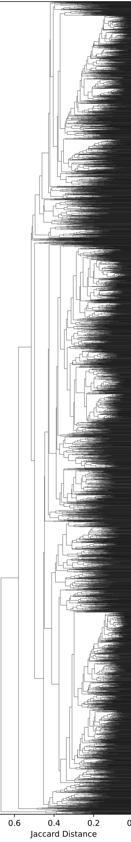
Hierarchical Clustering (5,000 bins, 30,000 samples)
