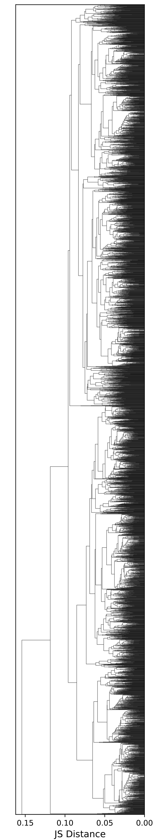
Hierarchical Clustering (5,000 bins, 50,000 samples)
