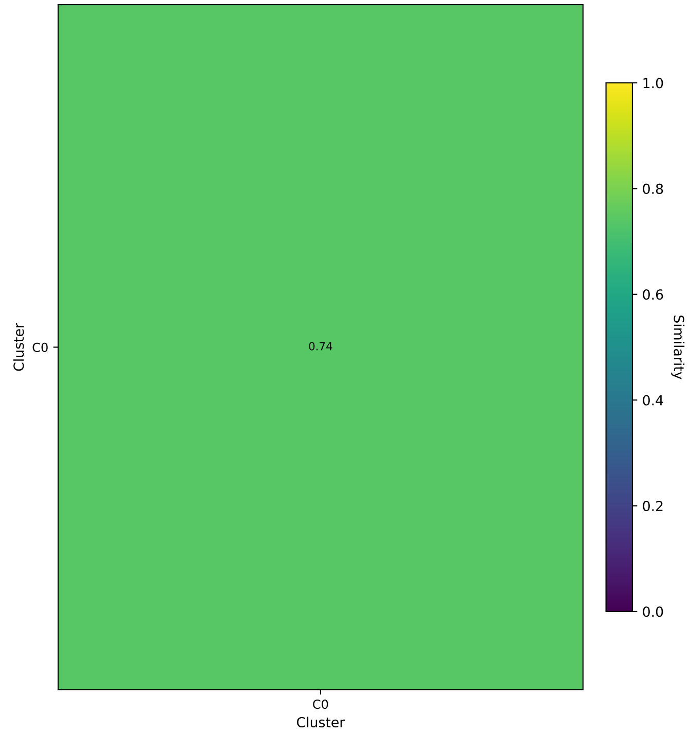
Inter-Cluster Similarity
