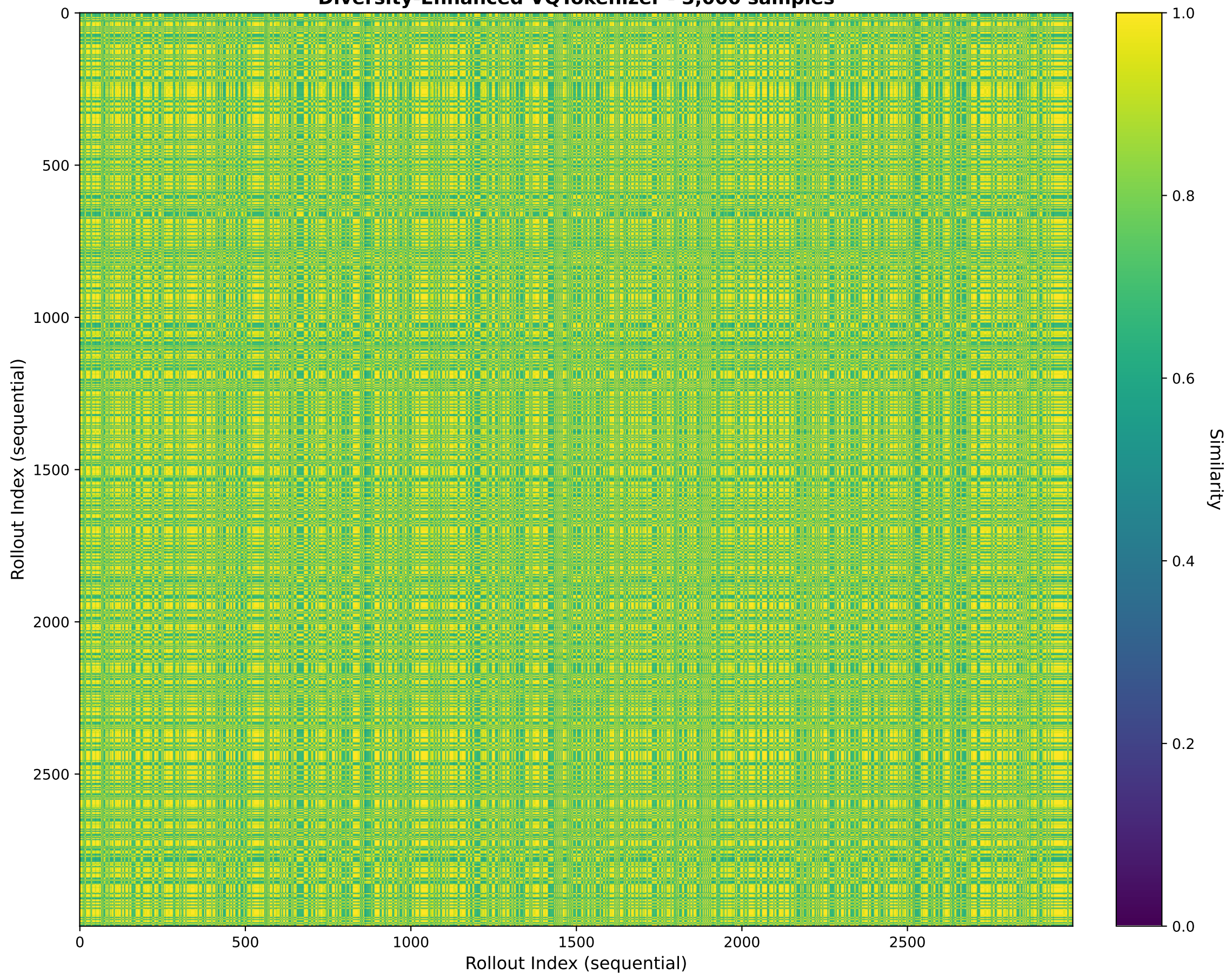
Rollout Token Similarity (Jaccard, All Families) Diversity-Enhanced VQTokenizer - 3,000 samples
