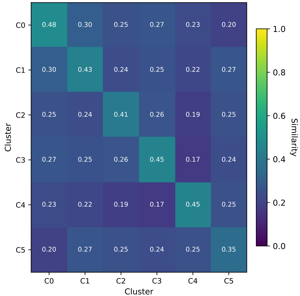
Inter-Cluster Similarity
