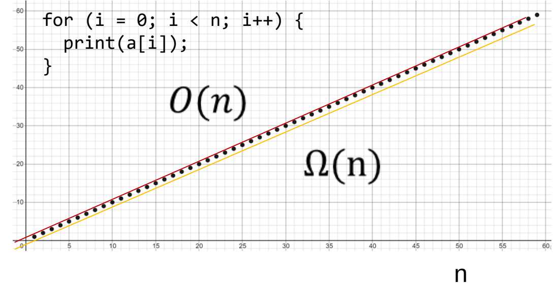
f(n) = n
