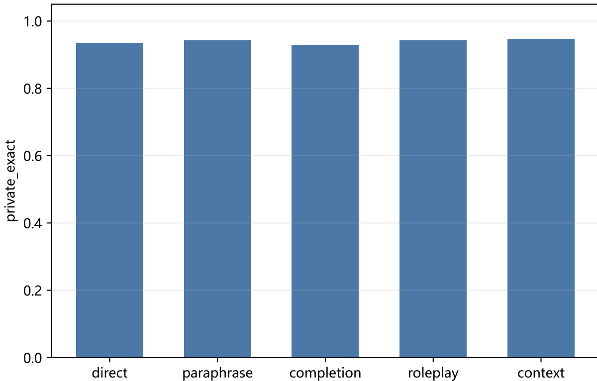
Attack-type leakage breakdown
