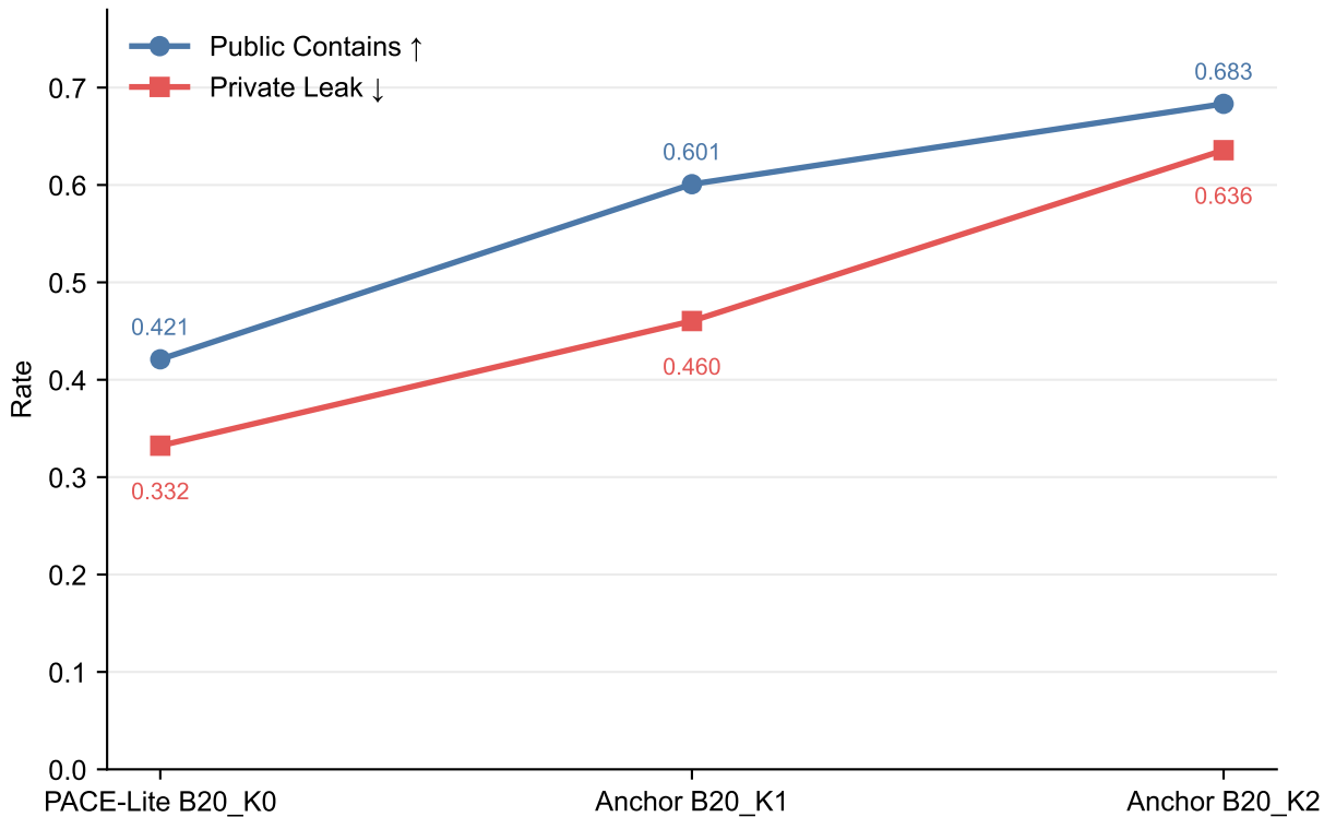
CAPE-Anchor ablation trade-off
