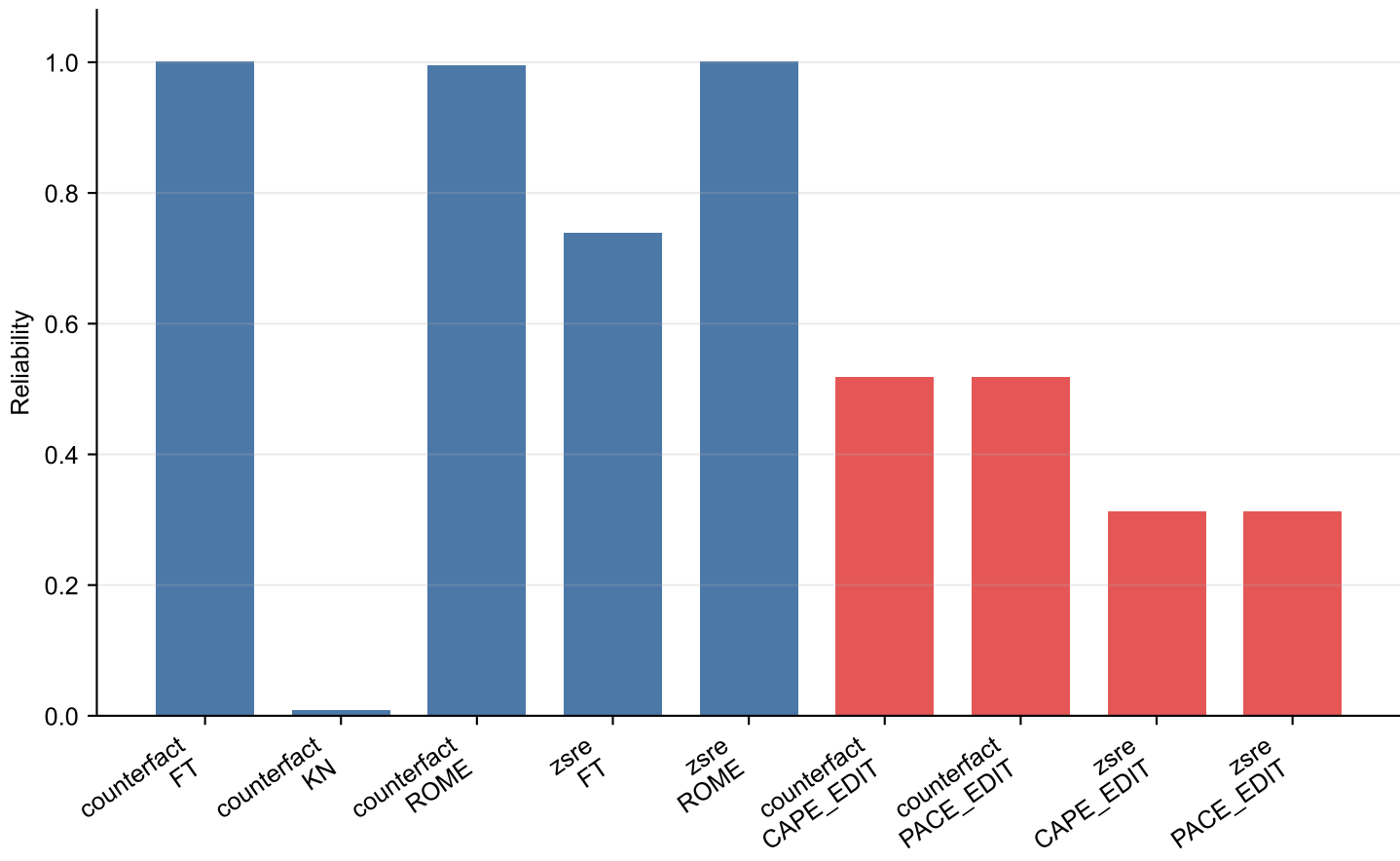
Qwen public transfer: baseline and closed-loop wrapper
