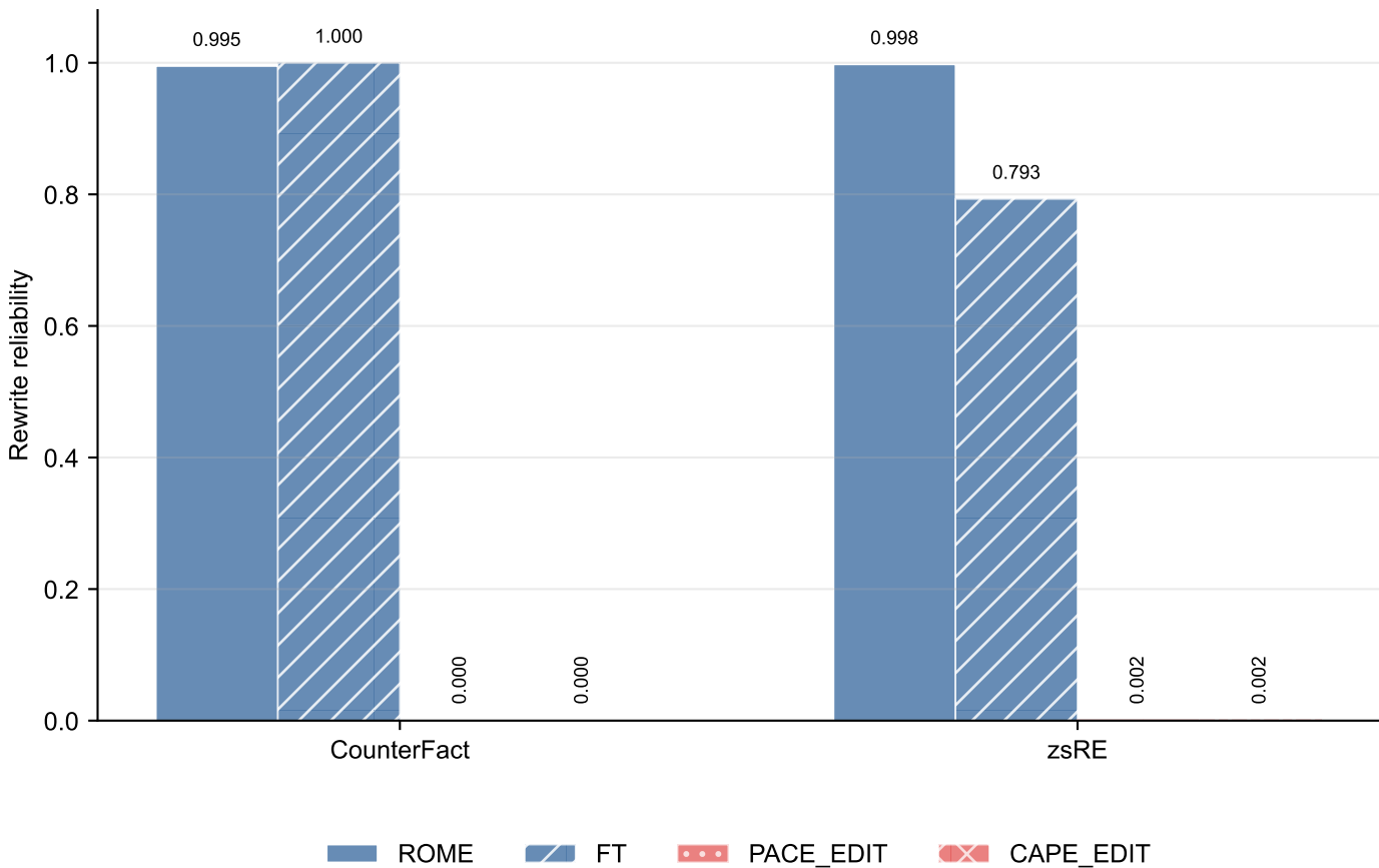
GPT-J Boundary Check: Baselines Remain Strong but Unretuned Wrappers Collapse
