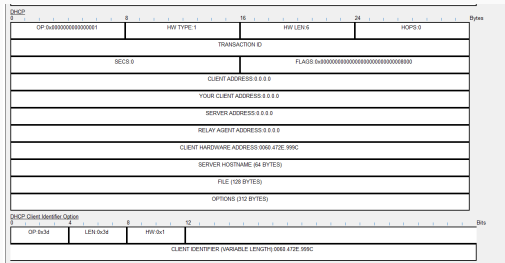
Рис. 9: DHCP Discover
