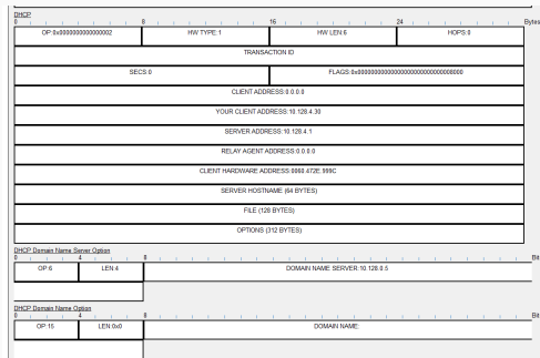
Рис. 10: DHCP Offer
