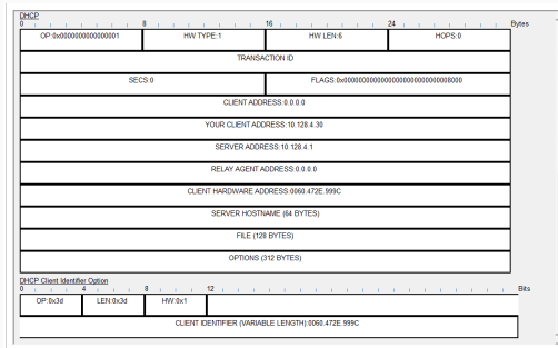
Рис. 11: DHCP Request
