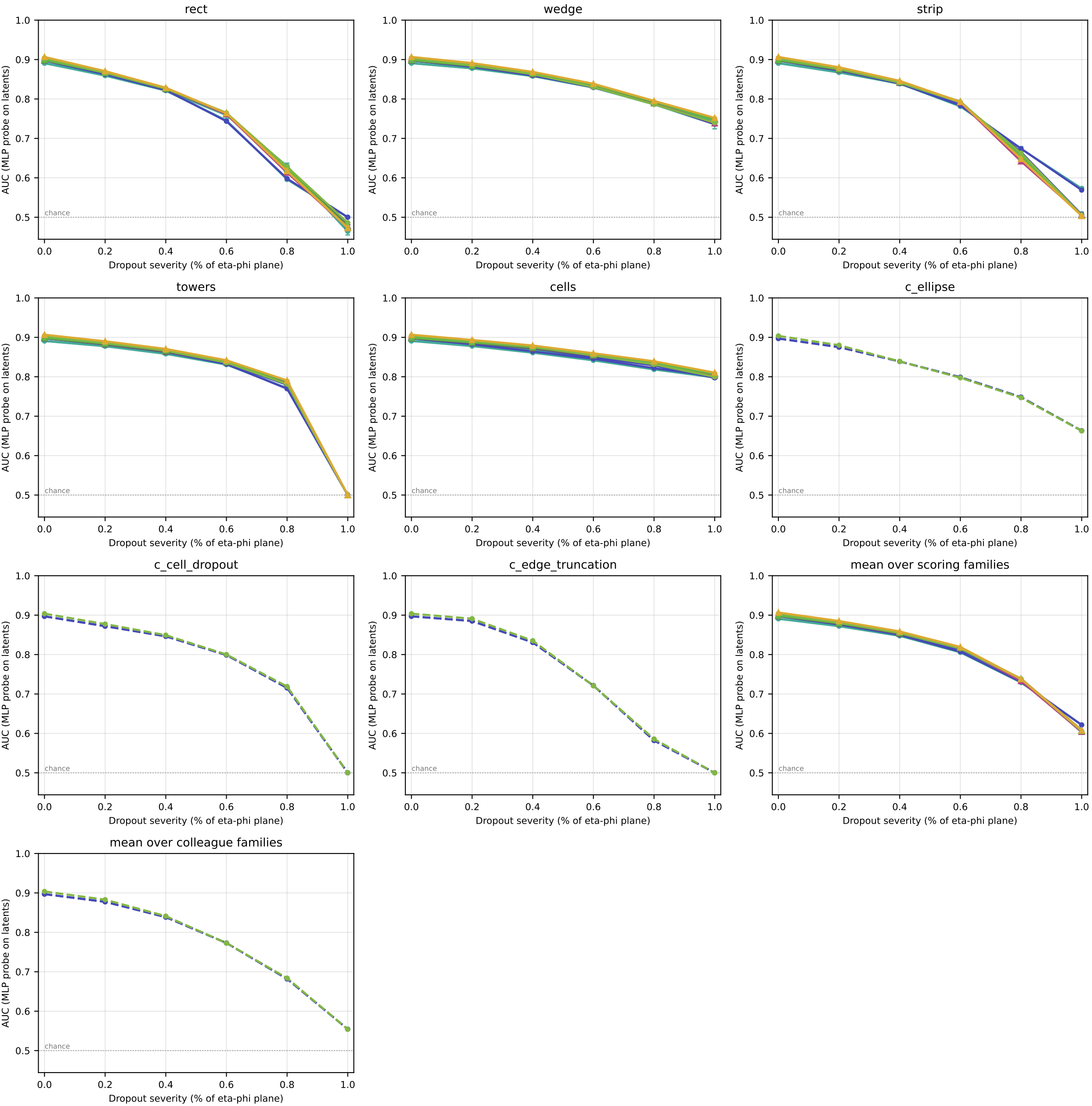
AUC vs severity on robust_tagging_eval_small_l1t.pt (L1T acceptance, eta in [-3, 3]) — not comparable to any area measured on the standard eval file
