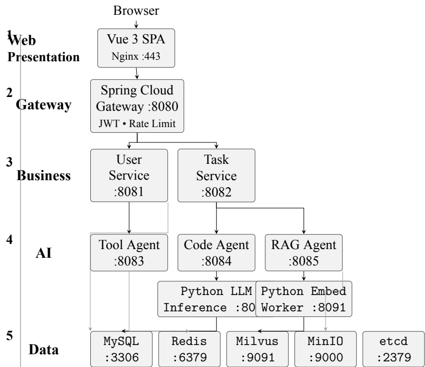
Figure 2: Five-Layer Architecture — Web, Gateway, Business, AI, and Data Layers with Internal Ports
