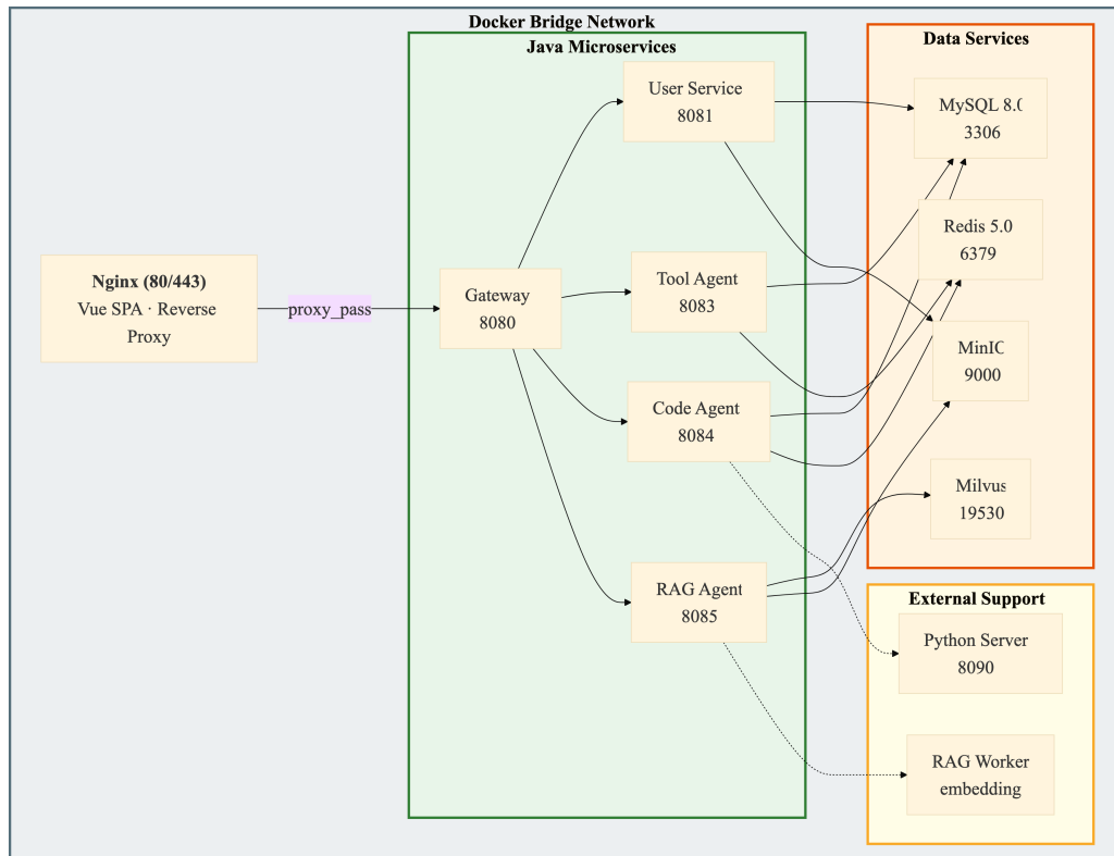
Figure 11: Figure 10: Docker Compose Service Topology
