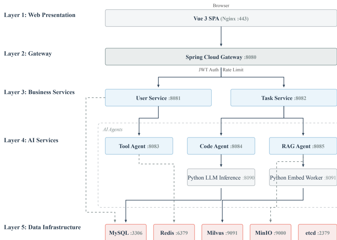
Figure 2: Five-Layer Architecture — All Services with Internal Ports
