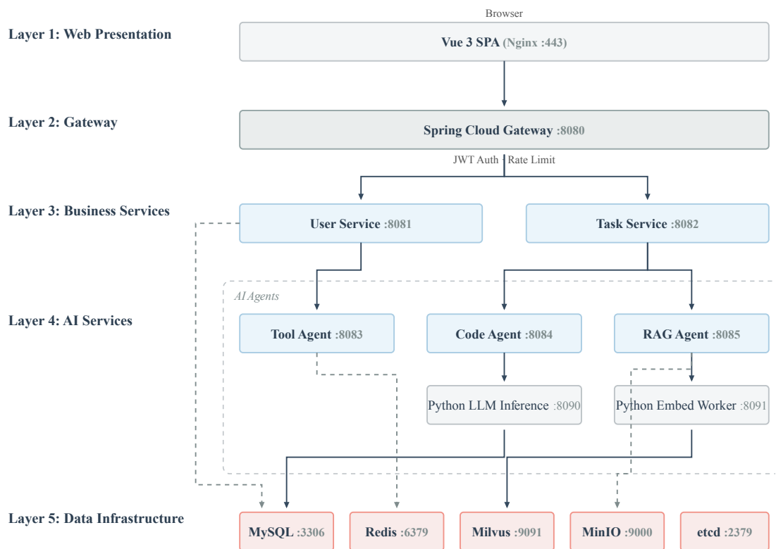
Figure 2: Five-Layer Architecture — All Services with Internal Ports
