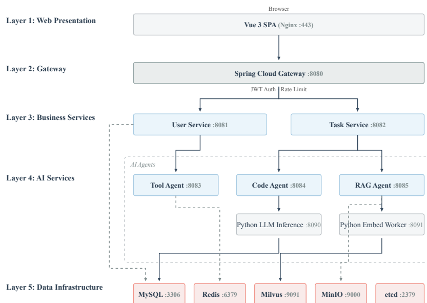
Figure 2: Five-Layer Architecture — All Services with Internal Ports
