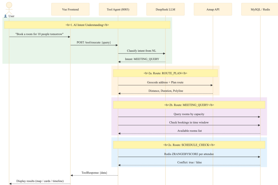
Figure 11: Copilot Query Flow — From Natural Language to Agent Execution
