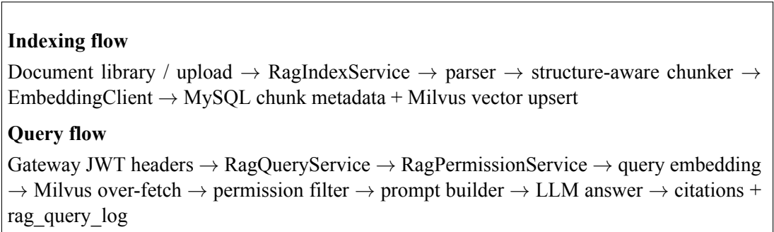
Figure 10: RAG Agent Architecture — Indexing Flow and Permission-Safe Query Flow
