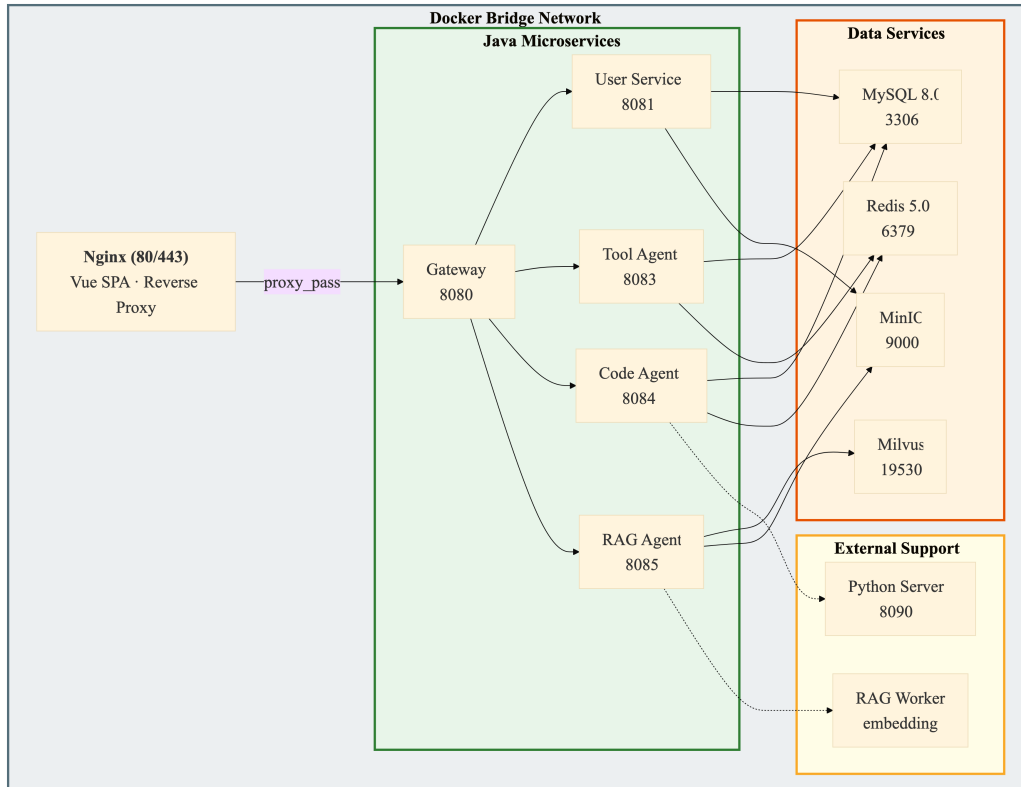
Figure 14: Docker Compose Service Topology
