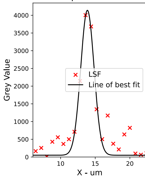
Line Spread Function
