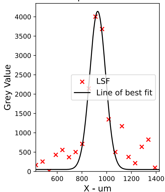
Line Spread Function
