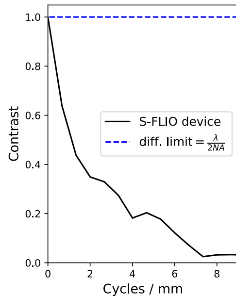
Modulation Transfer Function
