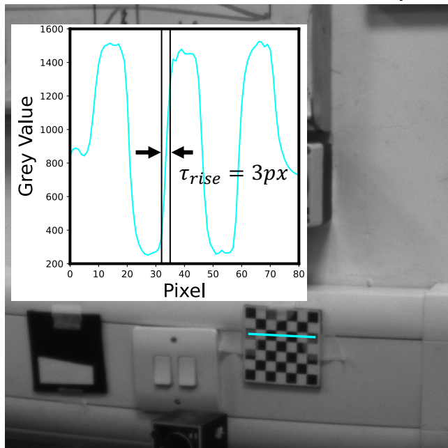
Brightfield without Beamsplitter
