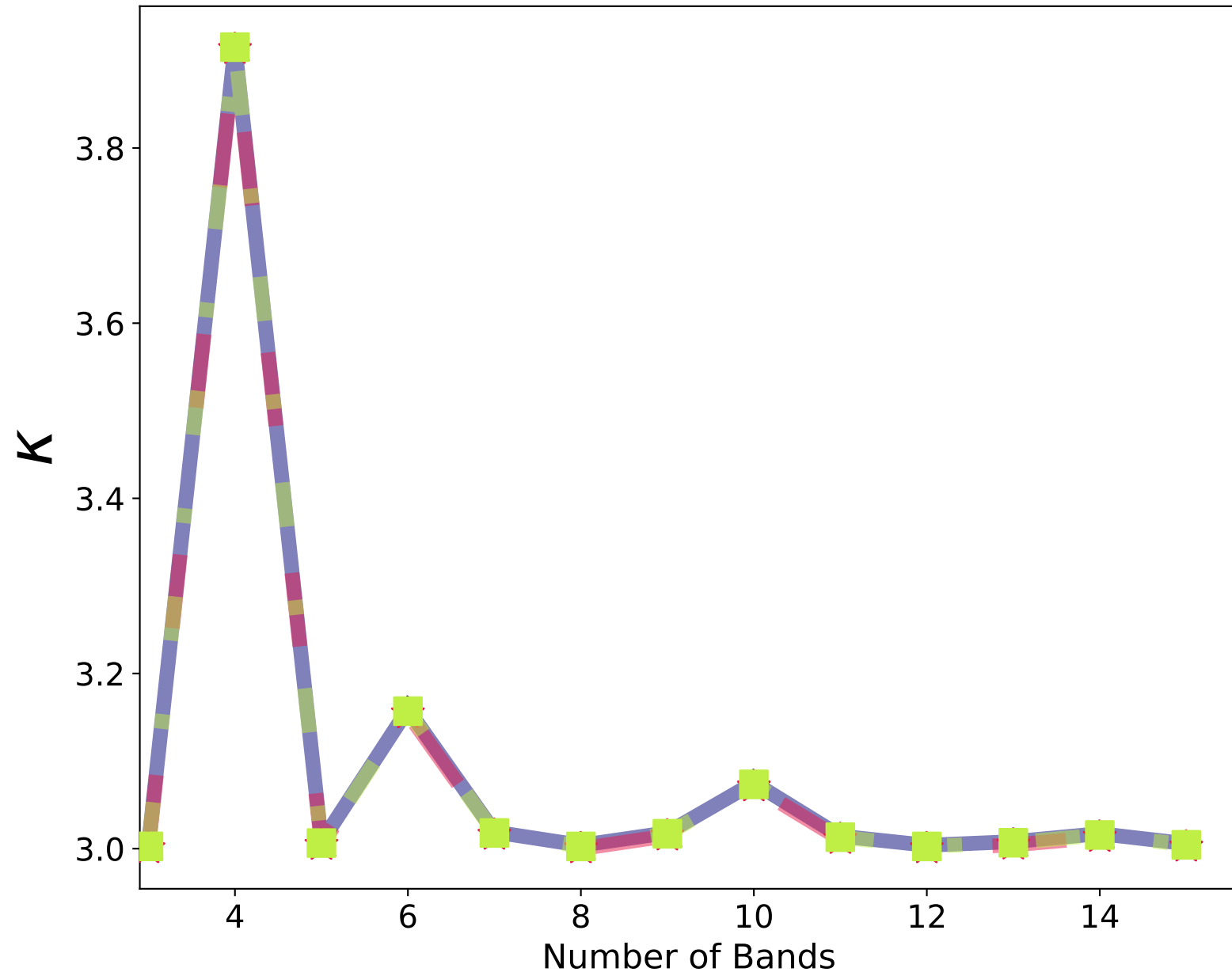
Condition Numbers
