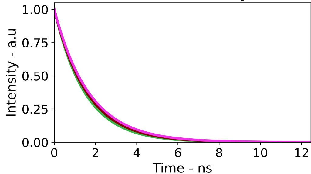
Endmember Decays
