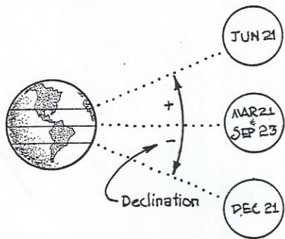
SOLAR DECLINATION
