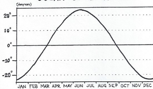
SOLAR DECLINATION
