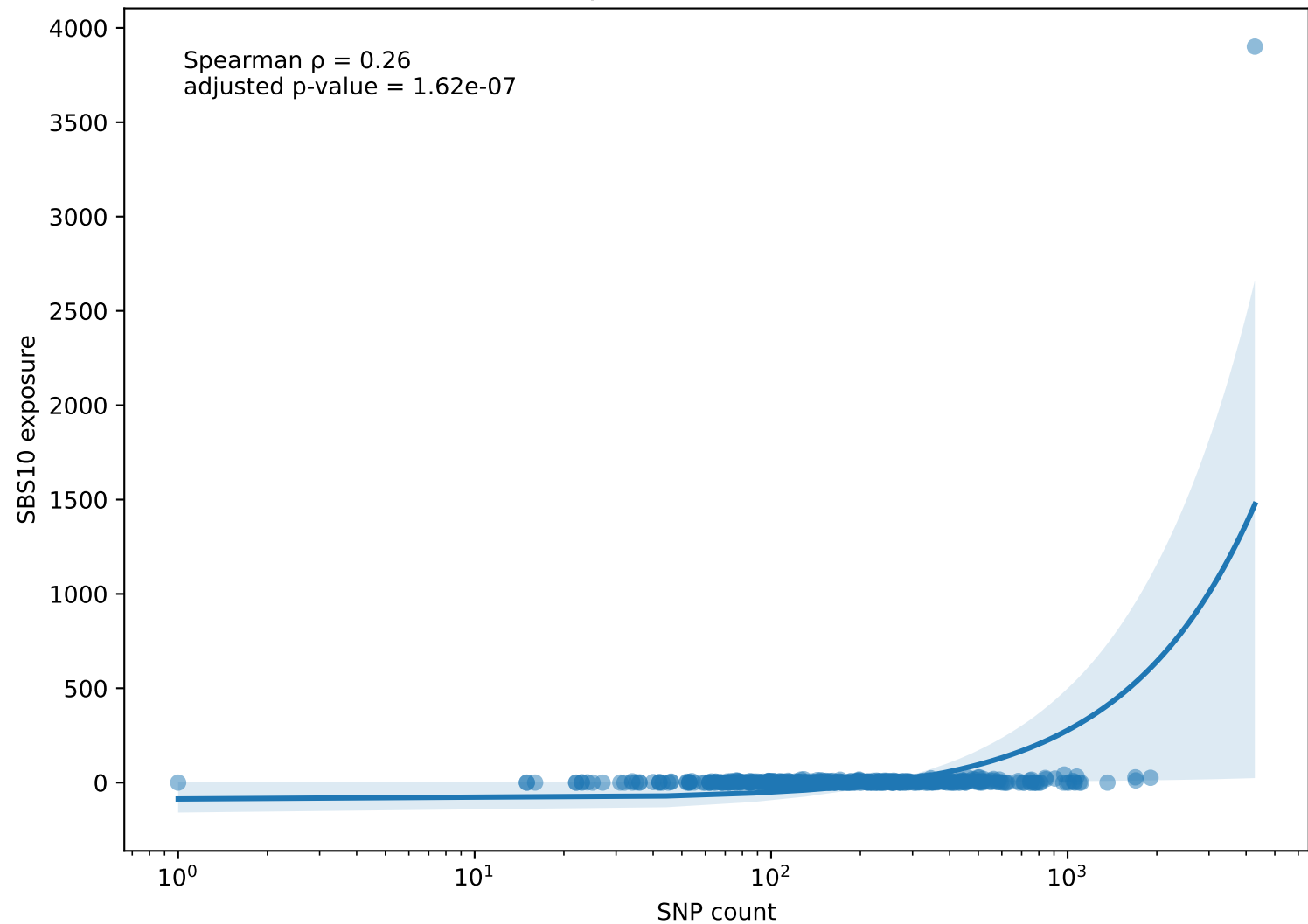
SBS10 exposure vs. mutation burden
