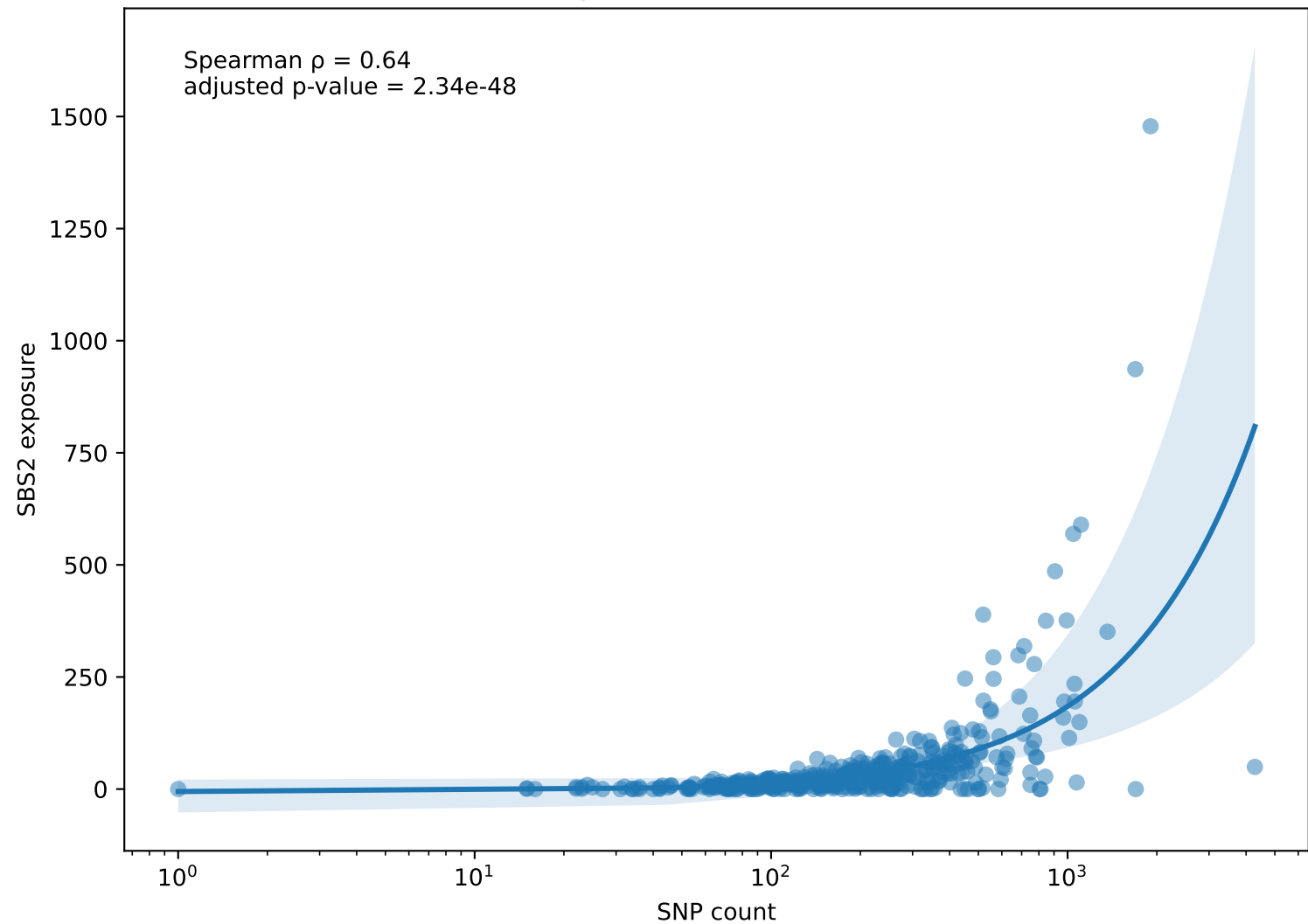
SBS2 exposure vs. mutation burden
