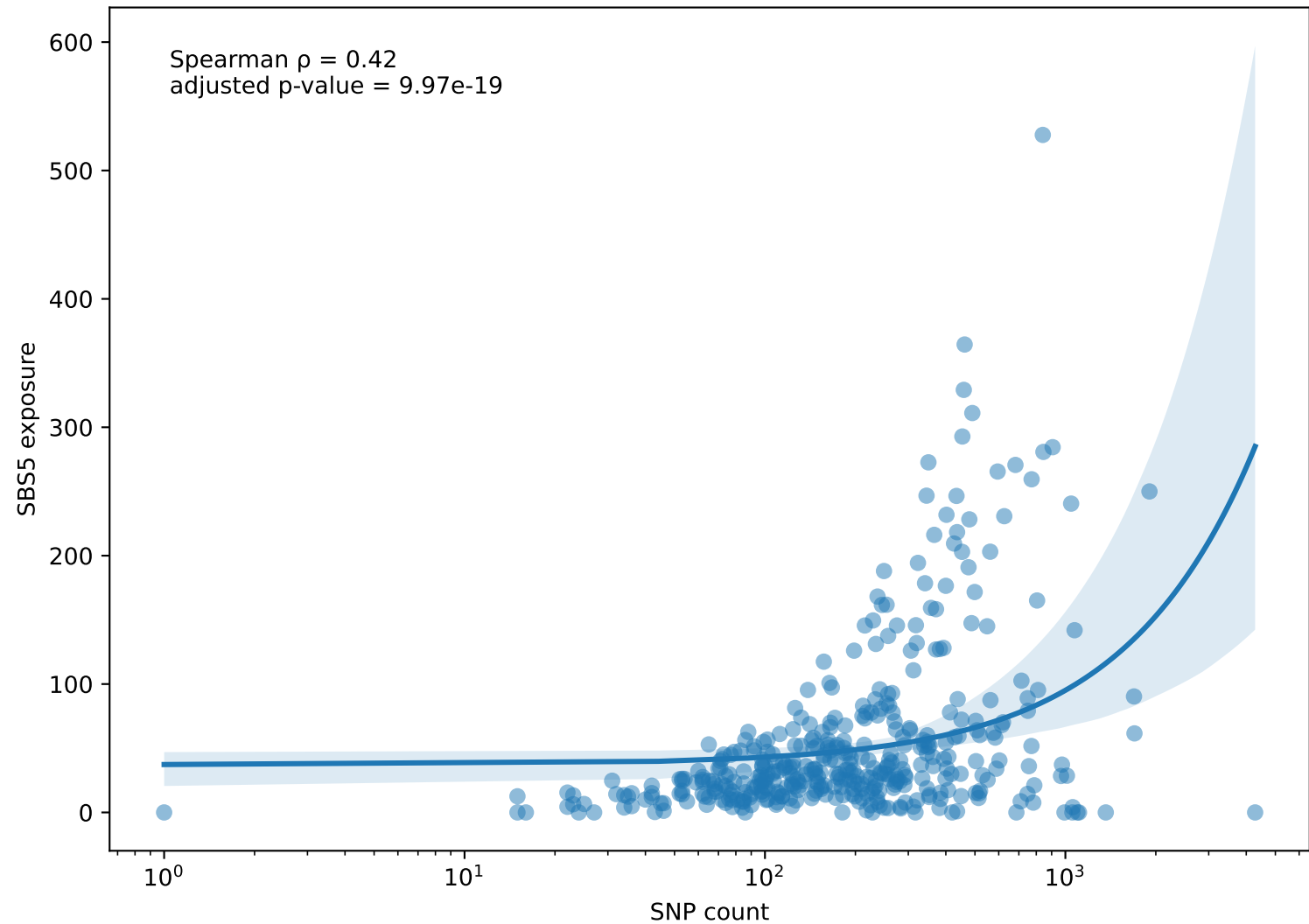
SBS5 exposure vs. mutation burden
