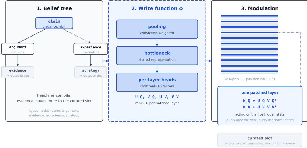
Figure 1: The three components in sequence. A typed belief tree (headline nodes compile; evidence leaves route to the curated slot) feeds the write function \phi (conviction-weighted pooling, a shared bottleneck, per-layer heads emitting rank-16 factors), which produces the U_Q, V_Q, U_V, V_V tensors patched into 11 of 32 layers. One patched layer, zoomed: the low-rank update acts on the live hidden state at both the query and value projections.
