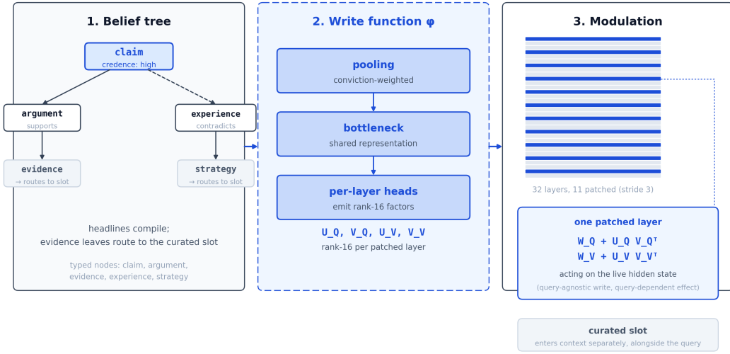
Figure 1: The three components in sequence. A typed belief tree (headline nodes compile; evidence leaves route to the curated slot) feeds the write function \phi (conviction-weighted pooling, a shared bottleneck, per-layer heads emitting rank-16 factors), which produces the U_Q, V_Q, U_V, V_V tensors patched into 11 of 32 layers. One patched layer, zoomed: the low-rank update acts on the live hidden state at both the query and value projections.
