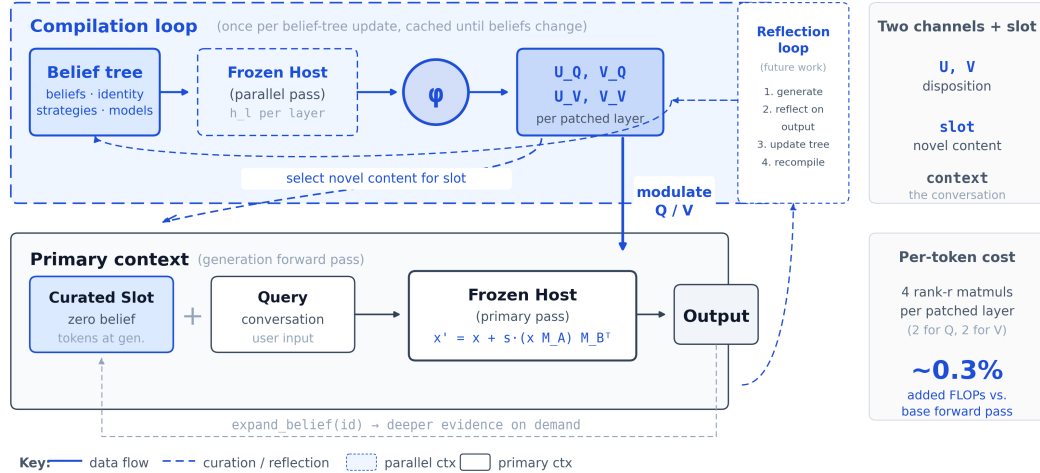
Figure 1: The three components in sequence. A typed belief tree (headline nodes compile; evidence leaves route to the curated slot) feeds the write function \phi (conviction-weighted pooling, a shared bottleneck, per-layer heads emitting rank-16 factors), which produces the U_Q, V_Q, U_V, V_V tensors patched into 11 of 32 layers. One patched layer, zoomed: the low-rank update acts on the live hidden state at both the query and value projections.
