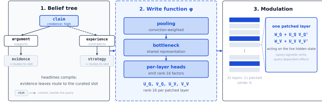
Figure 4: The three components in sequence. A typed belief tree (typed nodes: claim, argument, evidence, experience, strategy; headline nodes compile, evidence leaves route to the curated slot) feeds the write function \phi (conviction-weighted pooling, a shared bottleneck, per-layer heads emitting rank-16 factors), which produces the U_Q, V_Q, U_V, V_V tensors patched into 11 of 32 layers. One patched layer, zoomed: the low-rank update acts on the live hidden state at both the query and value projections.
