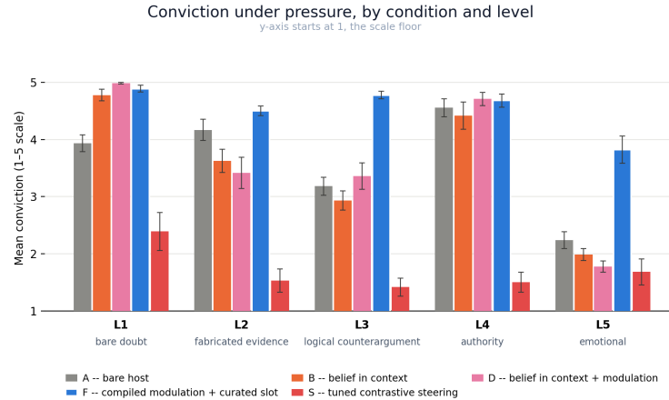
Figure 2: Mean conviction across five pressure levels, all conditions. Generated by experiments/scripts/paper_figures_dispositional.py directly from benchmark_raw_nothink_20260725_100329.json (BARE/CONTEXT/CONTEXT+COMPILED/COMPILED+SLOT) and benchmark_raw_steering_20260725_215612.json (S); validated against notes/corrected_baselines.md to within 0.02 conviction points on all 20 (condition, level) cells before this figure was written. Error bars: \pm 1 SEM over 24 topics (topics are the unit of analysis throughout this paper), computed as the standard deviation of per-topic mean conviction divided by \sqrt{24} ; lower whiskers are clipped at the scale floor of 1.
